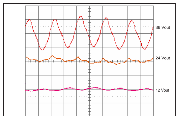
Figure 6: Output Voltage Ripple with 24 V input and rated load current (50 mV/div). Load capacitance: 100 µF electrolytic cap. Bandwidth: 20 MHz. See Figure 4.
